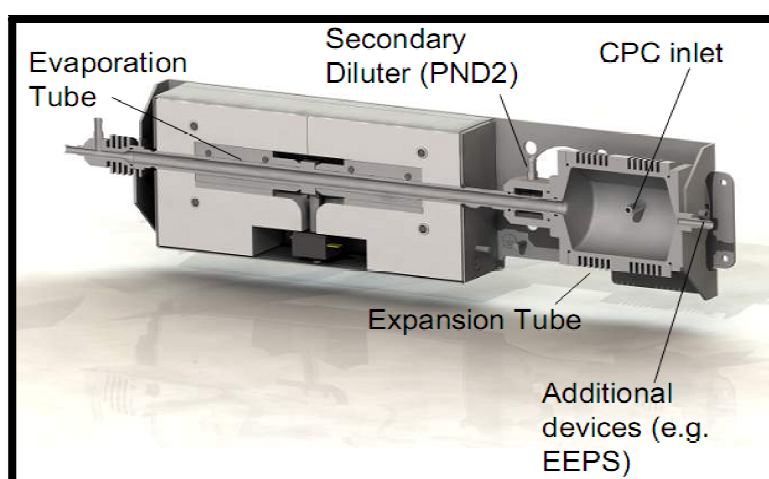
Fig4 (b): Particle number counter used during experiments sectional view [4]
