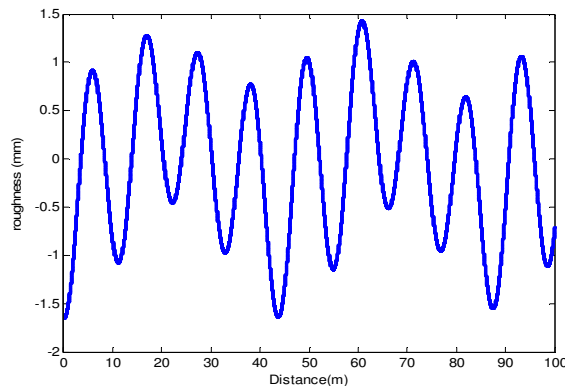
Fig3. Sample of the railway track irregularities
