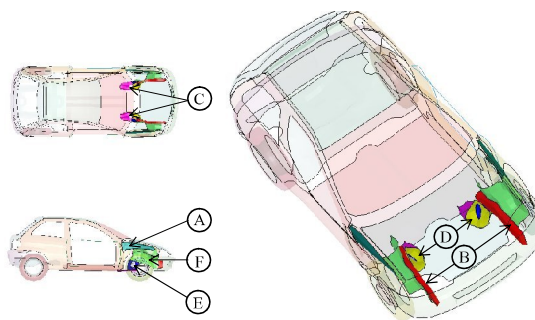
Fig. 4. Locations of design parameters within a transparent automotive body
