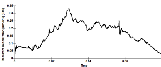
Fig. 6. Resultant deceleration versus time for the optimum condition design
