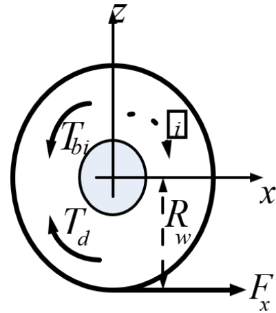
FIGURE 15: forces and the torques acting on the wheel
