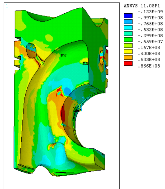
Fig. 10. Distribution of mean stresses in piston.
